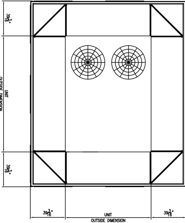
70" VERTICAL STYLE ENVISOR FOOTPRINT
