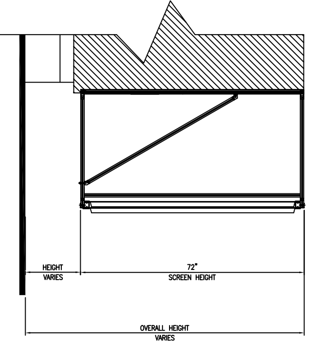
70" VERTICAL STYLE ENVISOR SECTION
