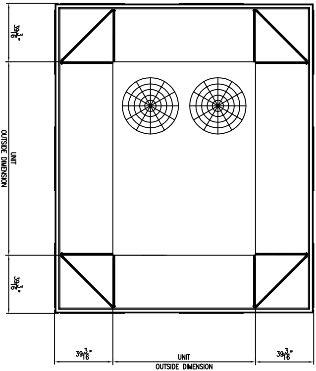
52" VERTICAL STYLE ENVISOR FOOTPRINT
