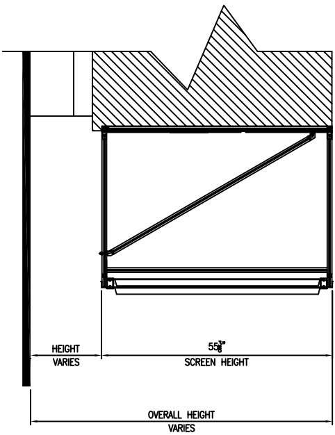
52" VERTICAL STYLE ENVISOR SECTION
