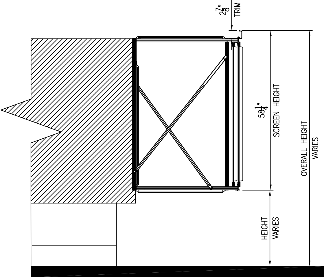
52" UNIT ATTACHED ENVISOR SECTION
