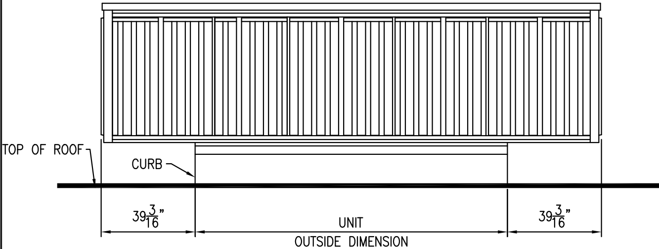
52" UNIT ATTACHED ENVISOR ELEVATION
