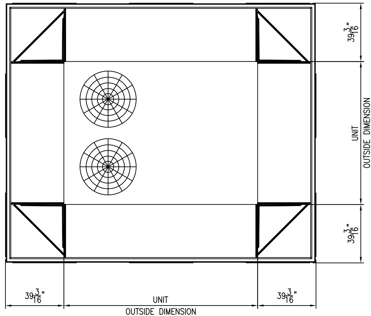
35" UNIT ATTACHED ENVISOR FOOTPRINT
