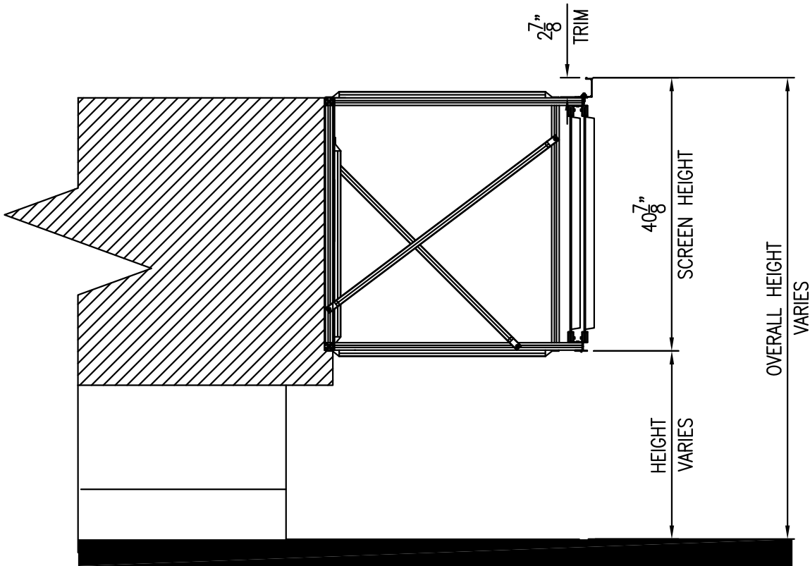
35" UNIT ATTACHED ENVISOR SECTION
