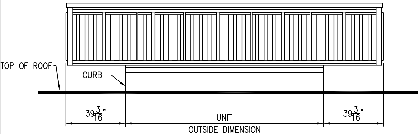
35" UNIT ATTACHED ENVISOR ELEVATION
