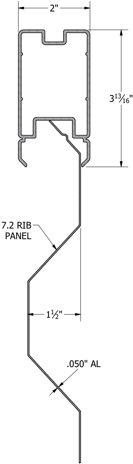
DETAIL B
