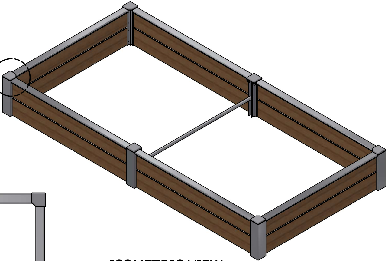
ISOMETRIC VIEW
