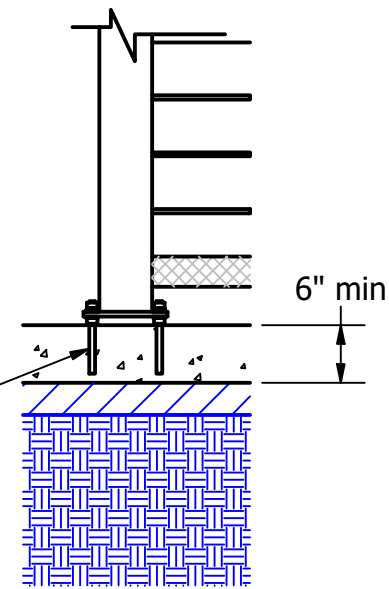
Post Anchor Attachment
