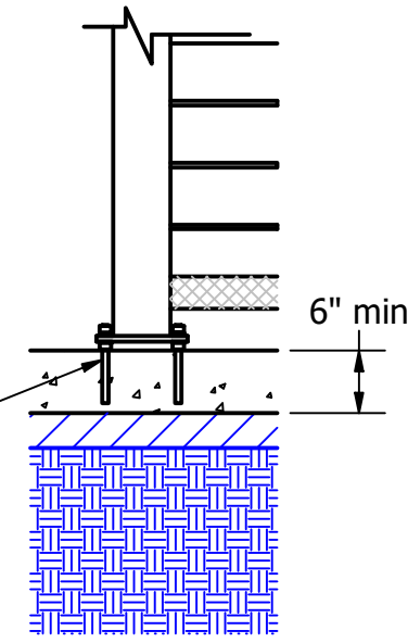
Post Anchor Attachment
